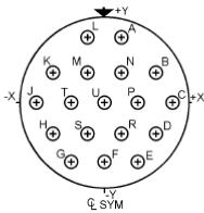
Contact Layout
