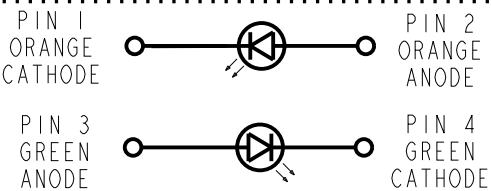
LED SCHEMATIC
