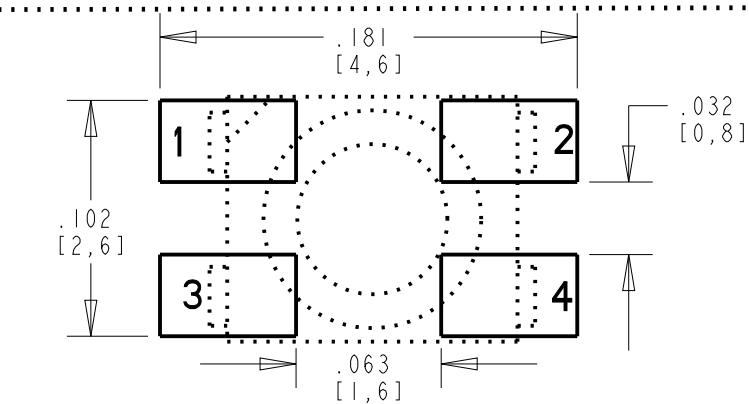
RECOMMENDED SOLDER PAD LAYOUT
