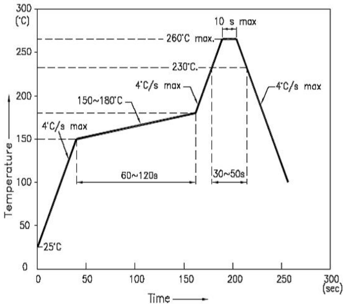
RECOMMENDED RoHS SOLDER PROFILE
