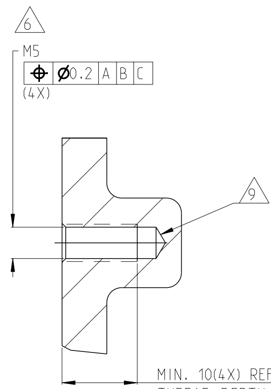
SECTION B-B
