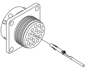
Contact Insertion - Ringlock
