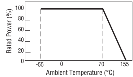
Derating Curve
