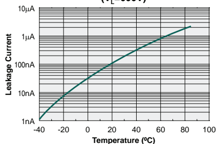
Typical Leakage vs. Temperature Measured Across Pins 1&2 ( V_L=600\text{V} )
