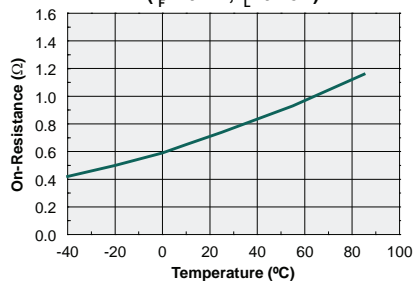
Typical On-Resistance vs. Temperature ( I_F=20\text{mA} , I_L=0.75\text{A} )
