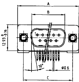
Plug connector
