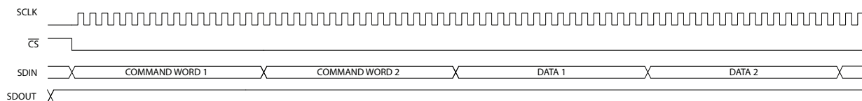
Figure 4-21: GSPI Write Timing—Auto-Increment with GSPI Link Disable Operation
