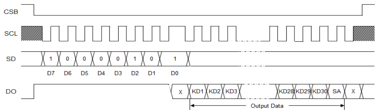
Figure 9. Serial Data Output
