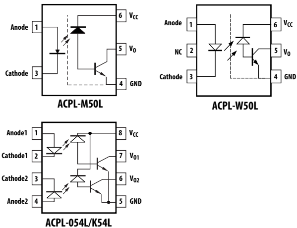
Figure 1: Functional Diagram
