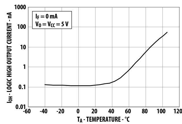
Figure 11: Typical Logic High Output Current vs. Temperature
