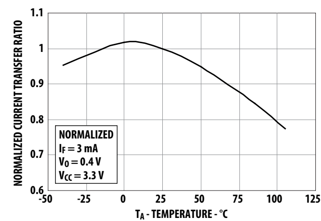
Figure 8: Typical Current Transfer Ratio vs. Temperature
