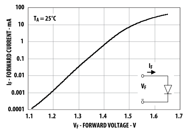
Figure 7: Input Current vs. Forward Voltage
