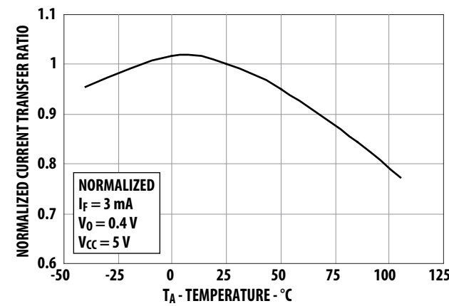
Figure 9: Typical Current Transfer Ratio vs. Temperature
