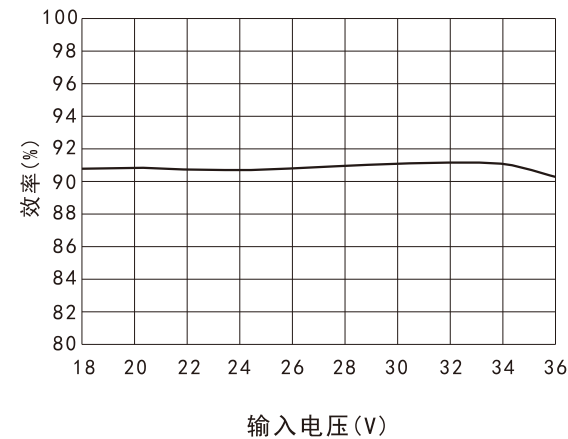
VRB2405YMD-15WR3
