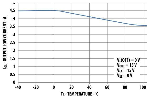
Figure 5: I_{OL} vs. Temperature
