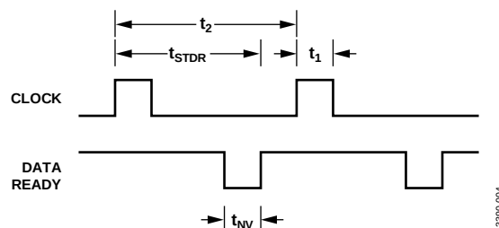
Figure 4. Input Clock Timing Diagram, \text{MSC\_CTRL}[0] = 1
