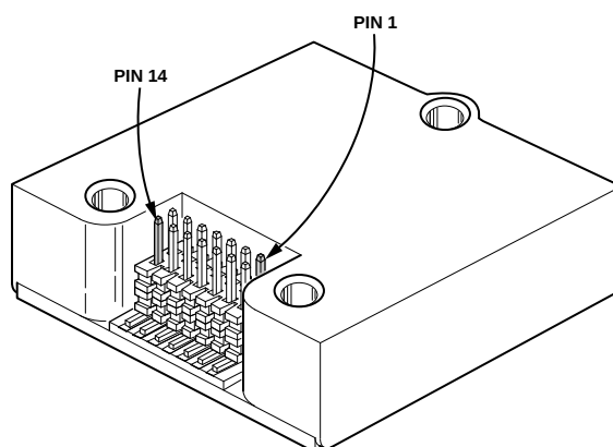
Figure 6. Pin Locations
