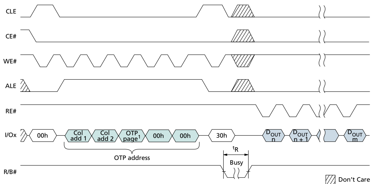
Figure 55: OTP DATA READ
