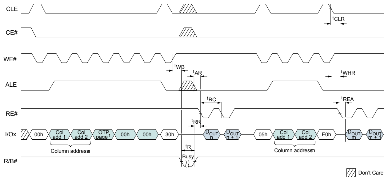
Figure 56: OTP DATA READ with RANDOM DATA READ Operation
