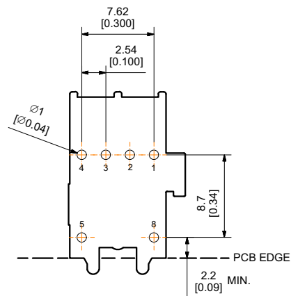
Figure 8 PCB Dimensions - Tilted (30°) Packages
