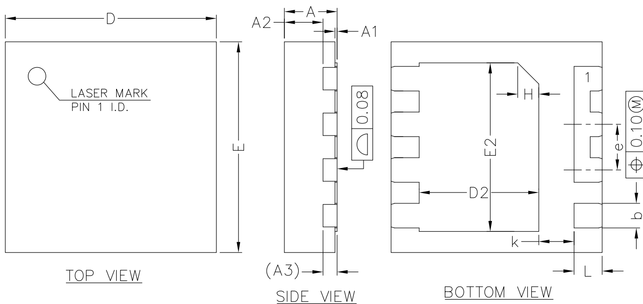
DFN3x3
