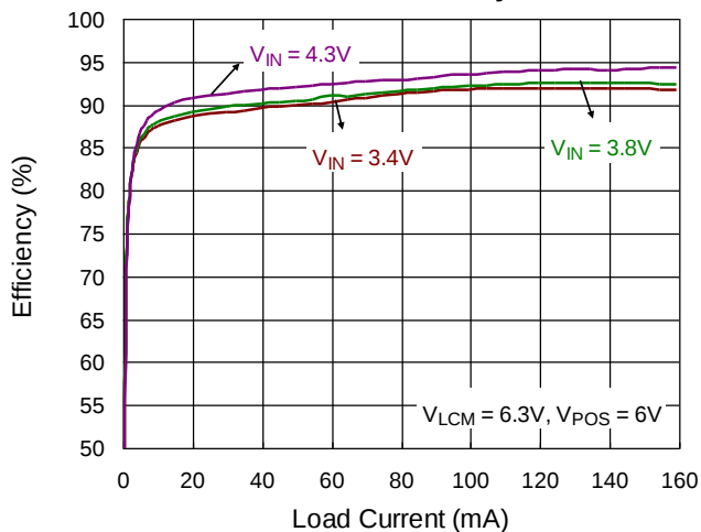
LCM Efficiency
