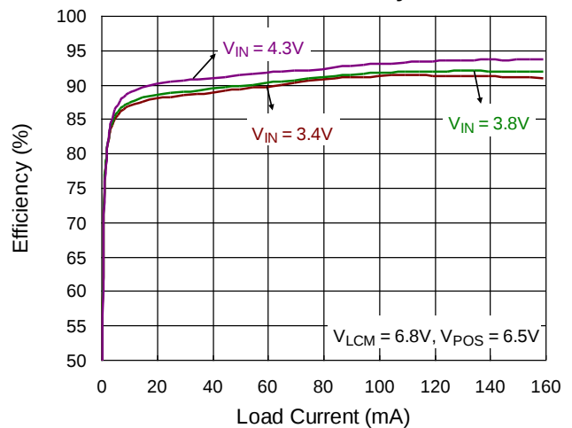
LCM Efficiency
