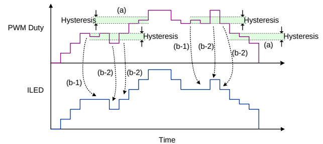
Figure 6. PWM Hysteresis
