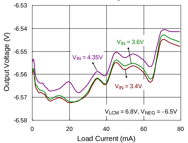
NEG Load Regulation
