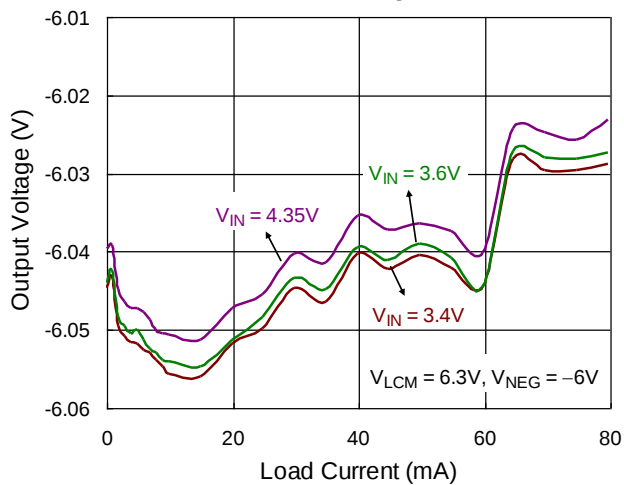
NEG Load Regulation
