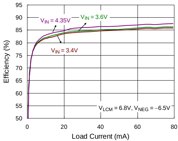
LCM+NEG Efficiency
