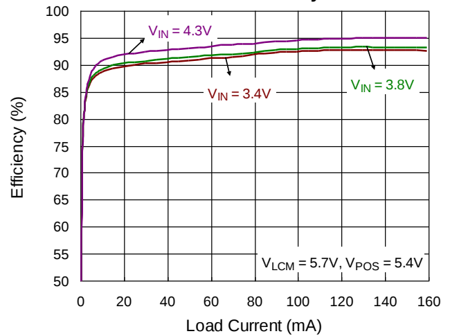
LCM Efficiency
