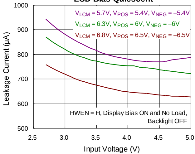
LCD Bias Quiescent
