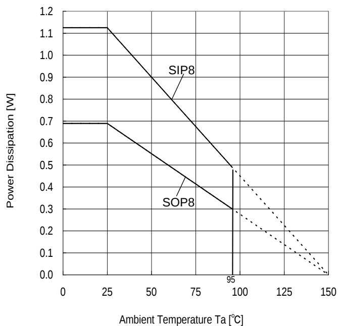
Figure 1 Derating curve
