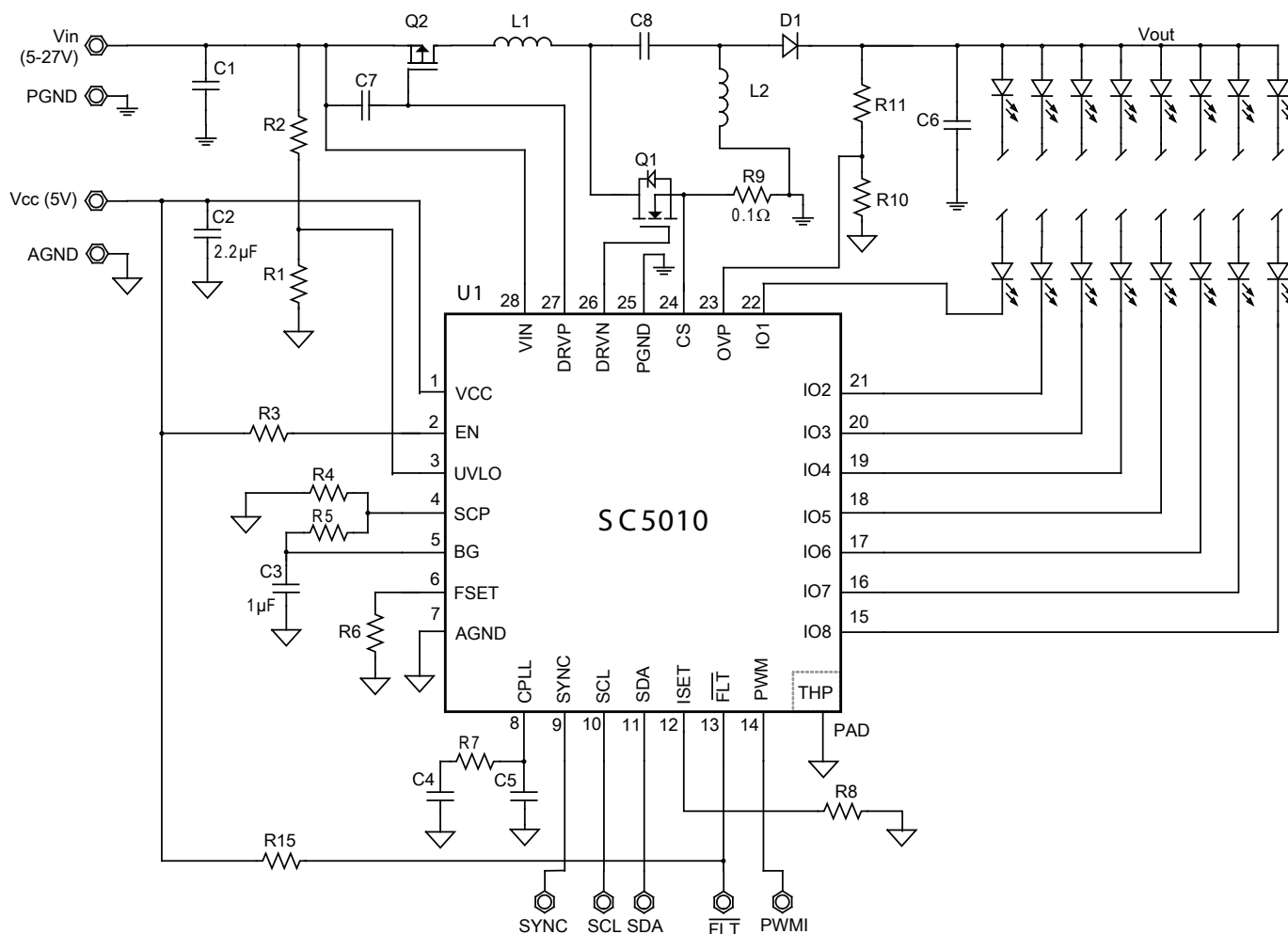
Figure 3 — SEPIC Configuration
