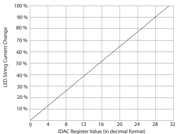
LED String Current Change vs. Analog Dimming Control Register (IDAC) Value
