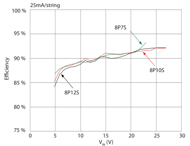
Backlight Efficiency vs. Input Voltage
