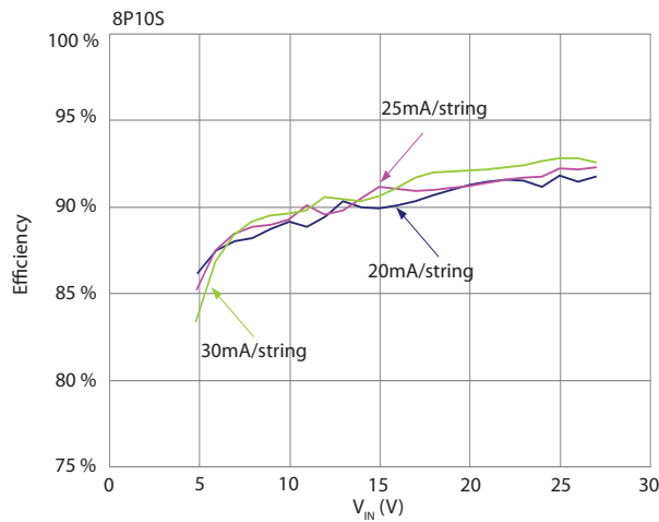
Backlight Efficiency vs. Input Voltage
