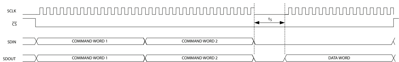
Figure 4-11: GSPI Read Timing—Single Read Access with Loop-Through Operation (default)
