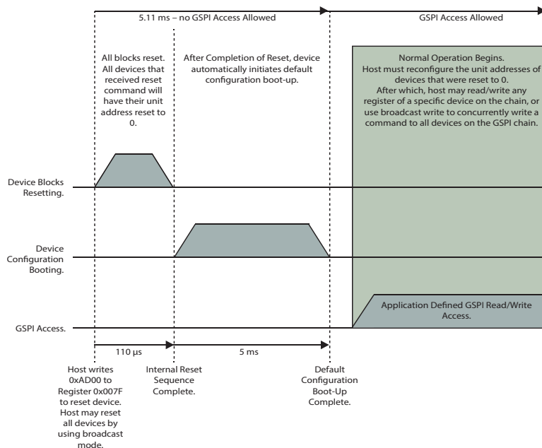
Figure 4-19: Power-Up Sequence.
