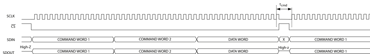
Figure 4-10: GSPI Write Timing—Single Write Access with Bus-Through Operation
