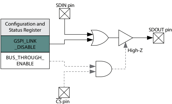
Figure 4-3: GSPI_LINK_DISABLE Operation
