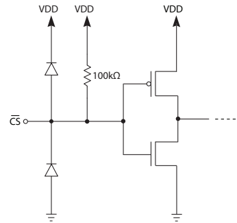
Figure 3-4: \overline{\text{CS}}
