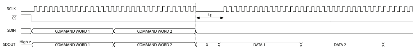
Figure 4-17: GSPI Read Timing—Auto-Increment Read with Bus-through Operation
