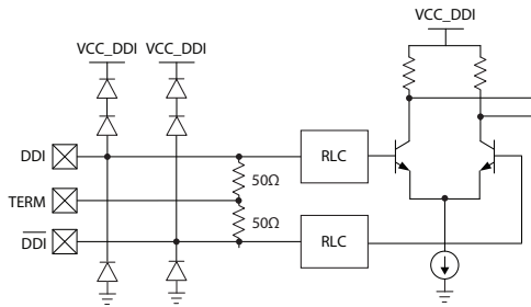
Figure 3-1: DDI, \overline{\text{DDI}}
