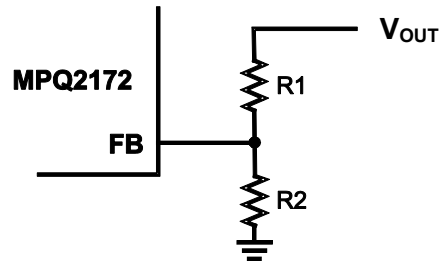
Figure 1: Feedback Circuit
