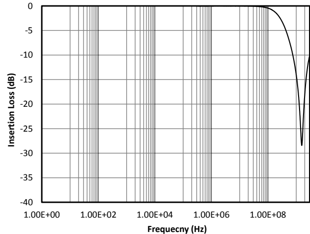
Insertion Loss
