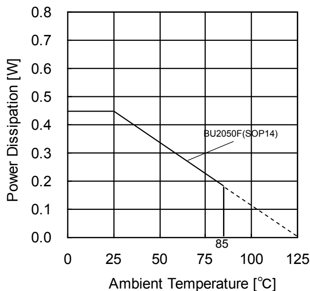
Figure 9. Derating Curve
