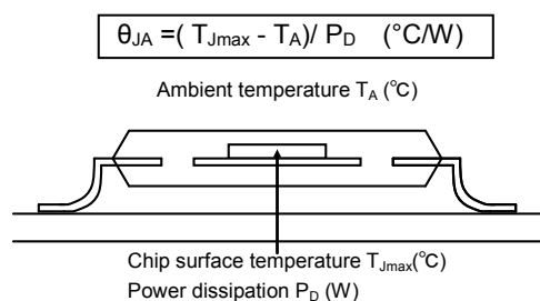
Figure 8. Thermal resistance
