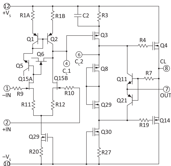
Figure 1: Equivalent Schematic
