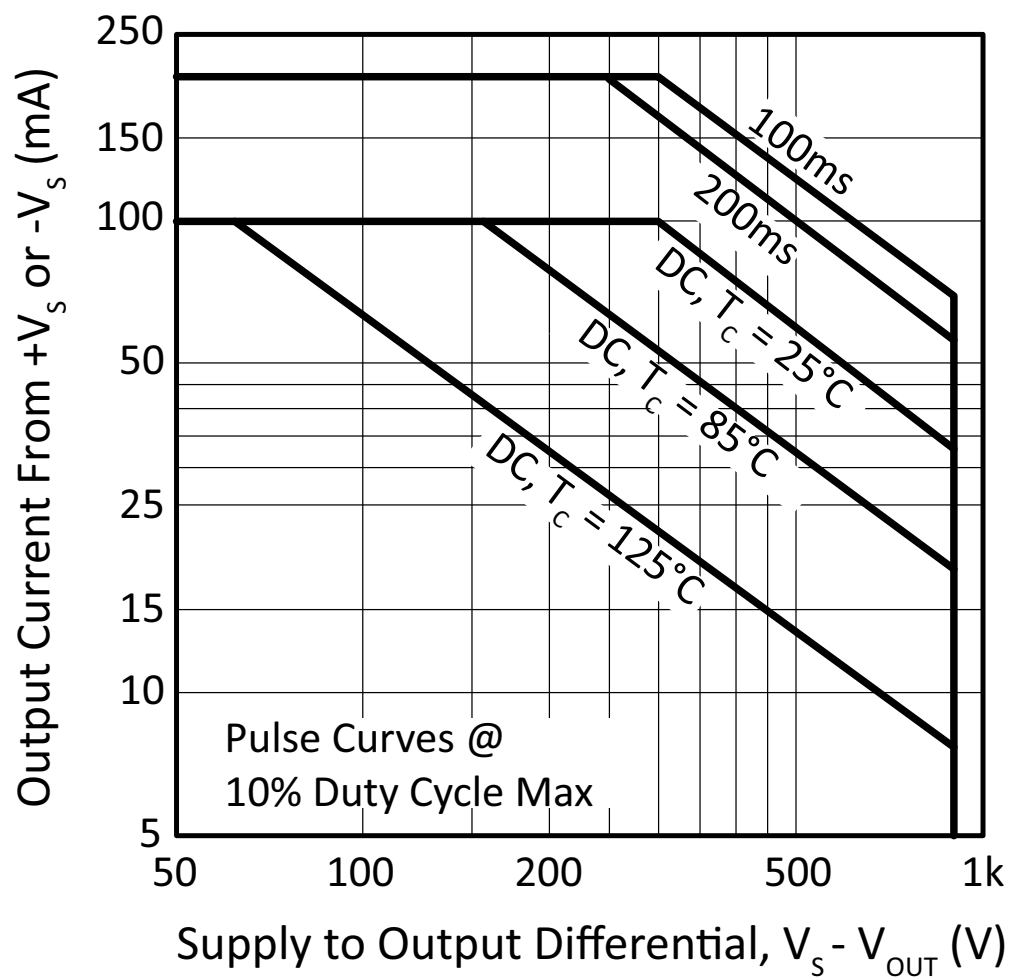
Figure 12: SOA
