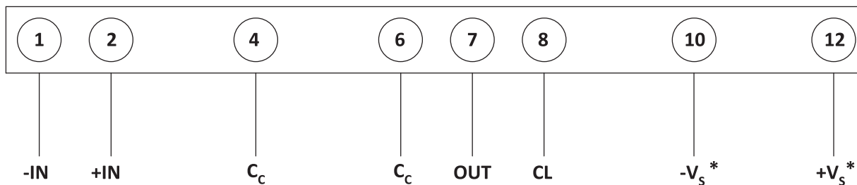
Figure 3: External Connections
