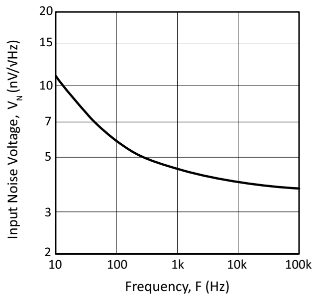
Figure 11: Input Noise
