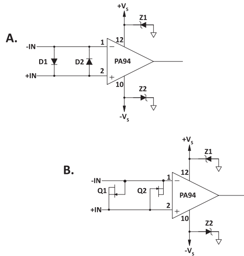
Figure 14: Overvoltage Protection
