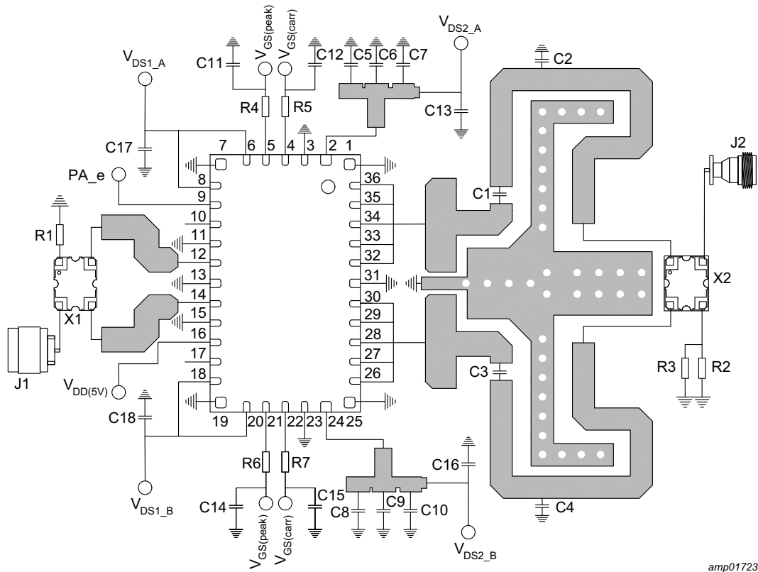
Fig 4. Electrical schematic
