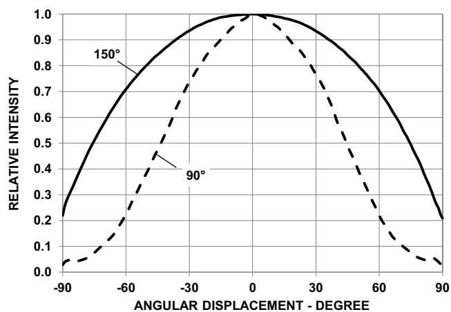
Figure 7: Radiation Pattern
