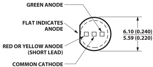
HLMP-40xx Straight Leads
