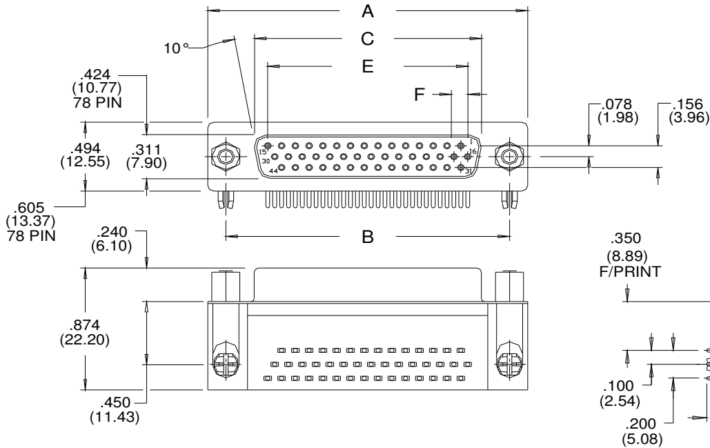
RECEPTACLE 634 SERIES
