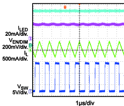
Minimum Analog Dimming
