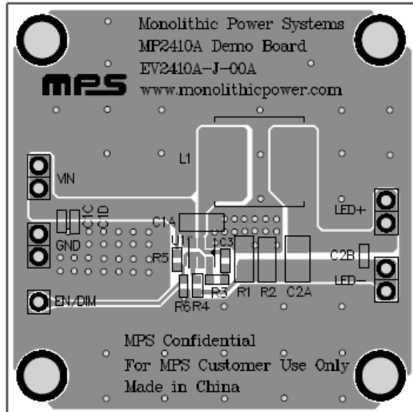
Figure 2 - Top Layer
