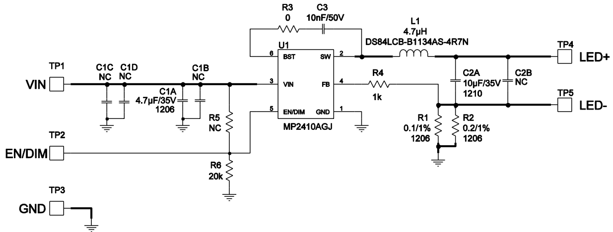
Figure 1 - Schematic
