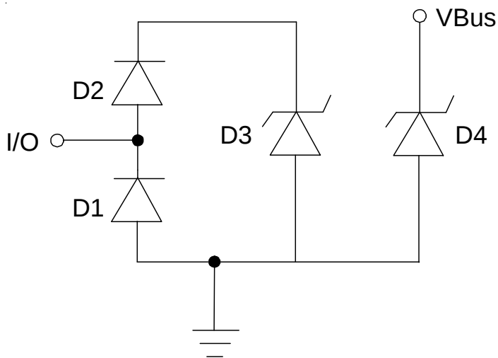
Spice Model
