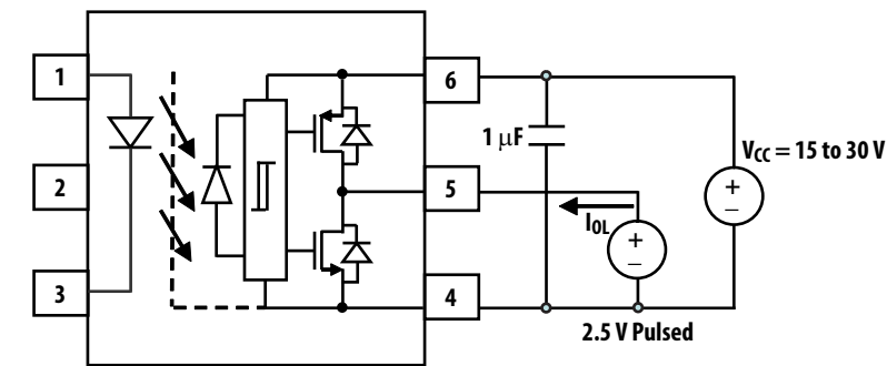
Figure 21 I_{OL} Test Circuit
