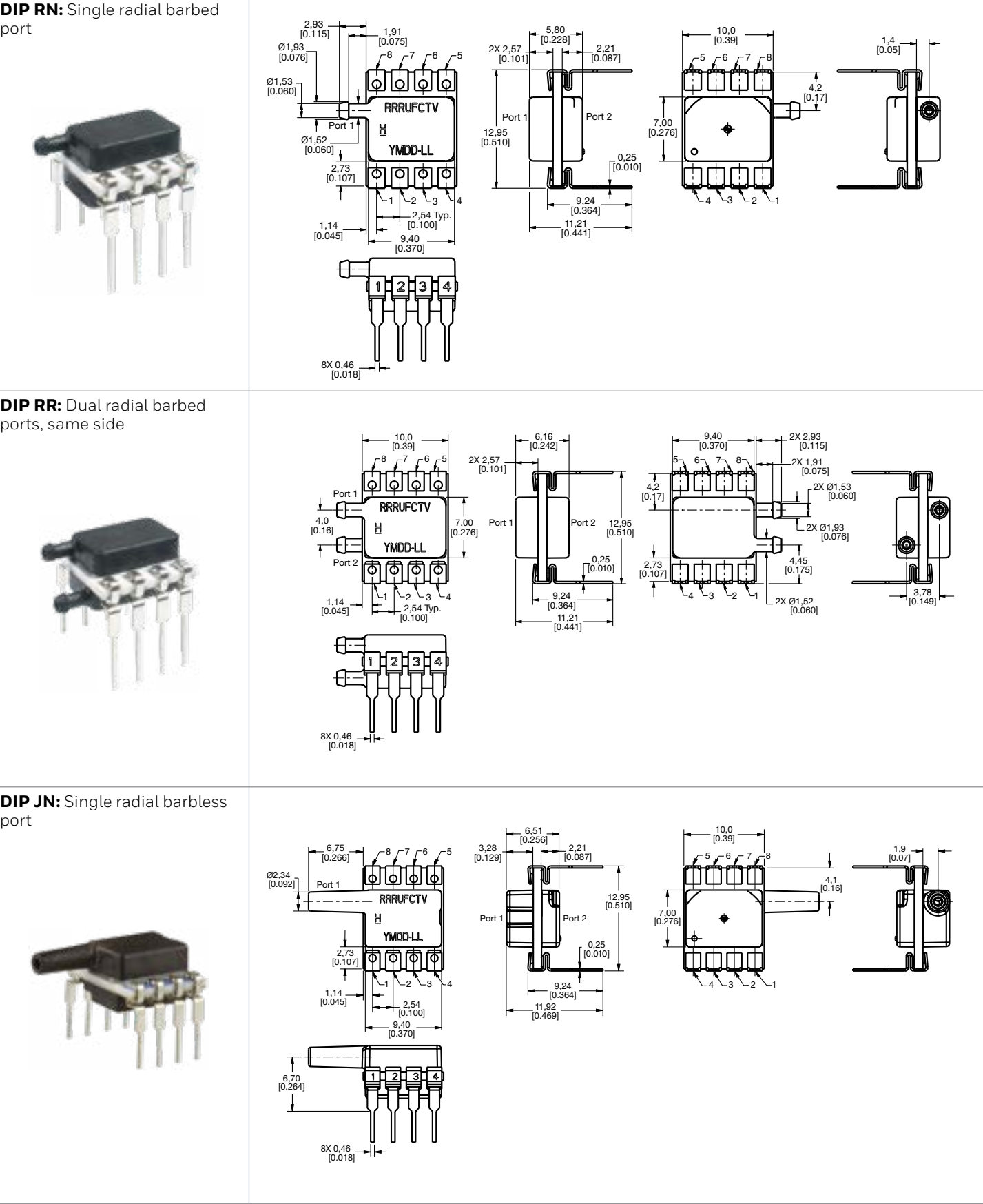
Figure 4. DIP Package Dimensional Drawings (continued)
