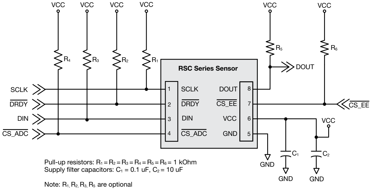
Figure 7. Recommended Circuit
