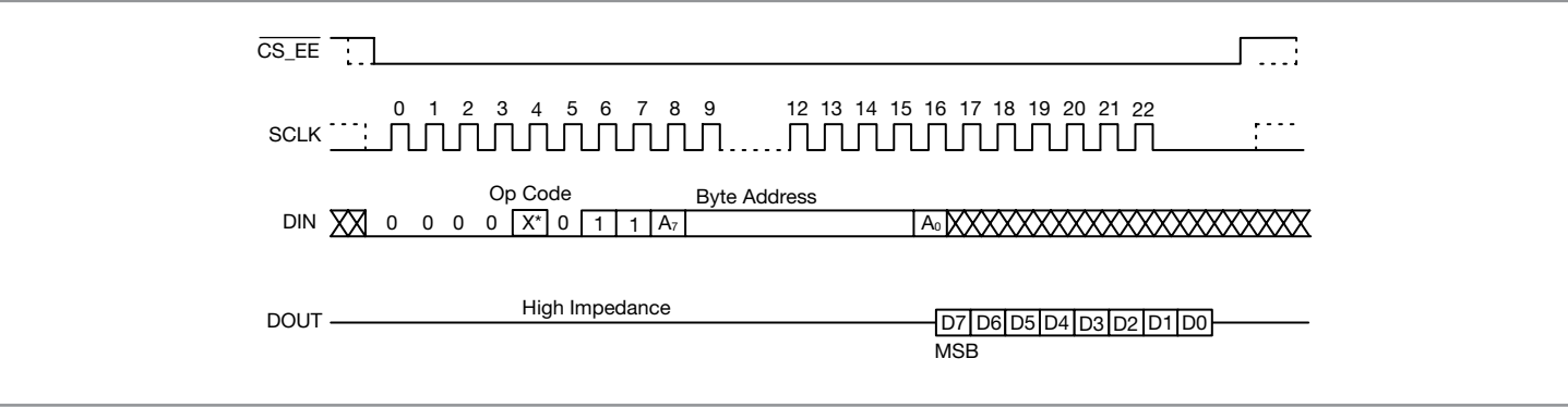
Figure 2-1. EEPROM Communications
