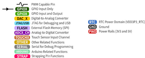
ESP32-C3-DevKitM-1 Pin Layout (click to enlarge)
