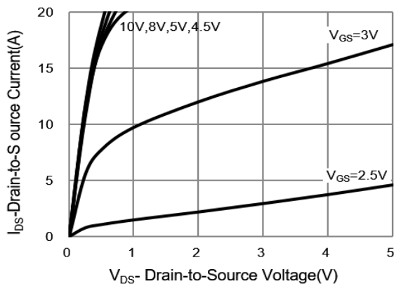
Fig.1 On-Region Characteristics
