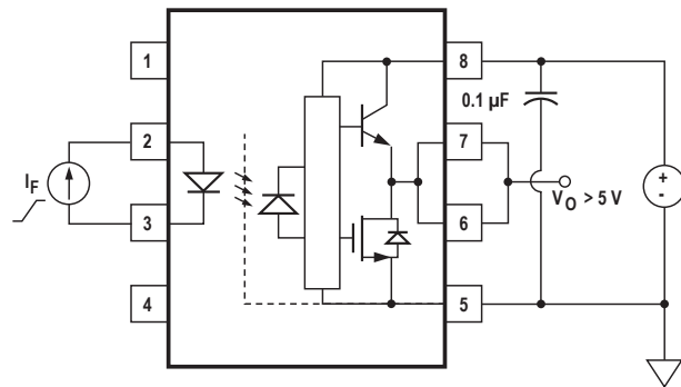
Figure 25. I_{FLH} Test Circuit.
