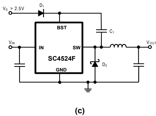
Figure 6(a)-(d). Methods of Bootstrapping the SC4524F
