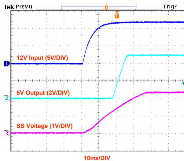
V_{IN} Start up Transient ( I_O=2A )
