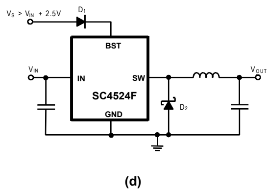
Figure 6(a)-(d). Methods of Bootstrapping the SC4524F
