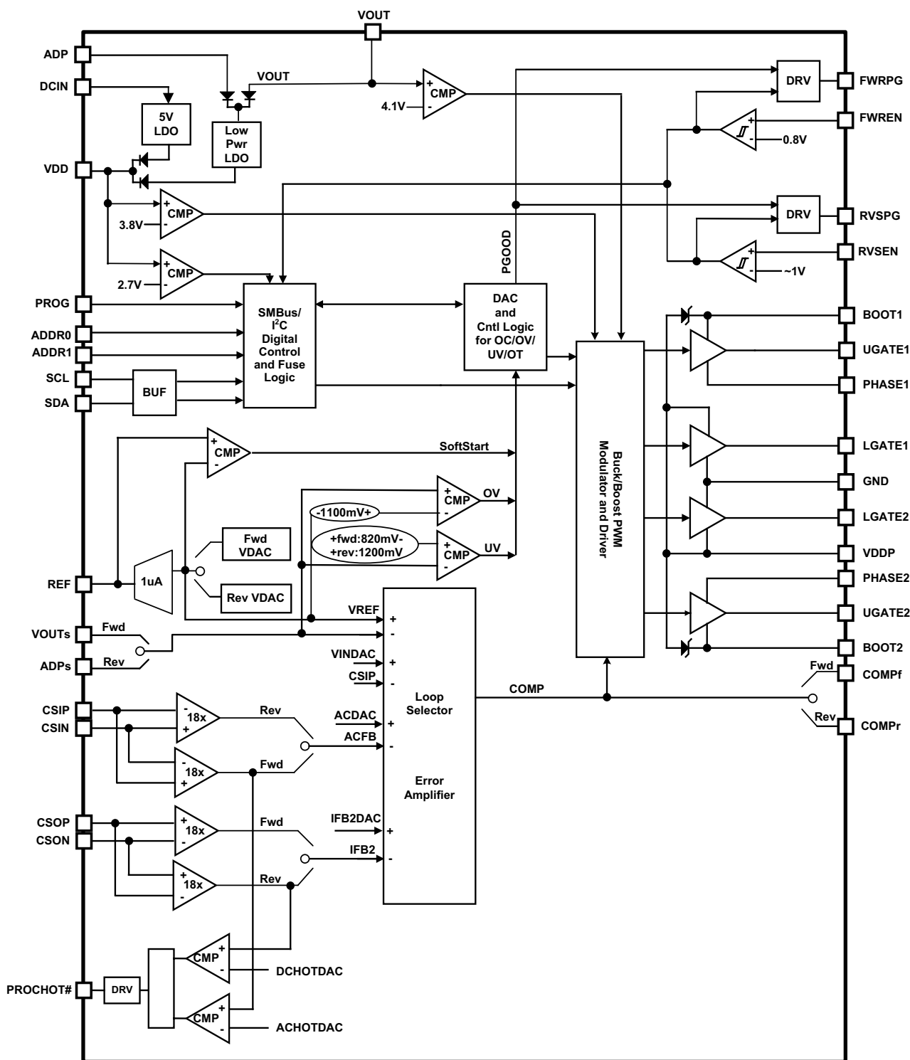
Figure 2. Block Diagram
