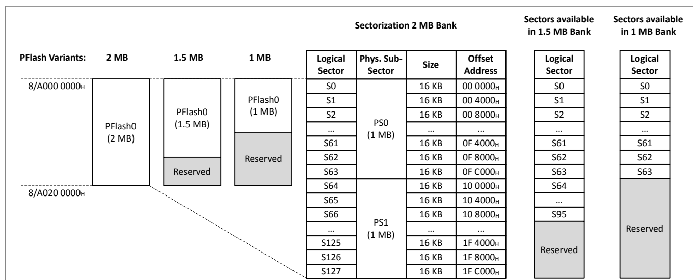
Figure 1 PFlash variants
