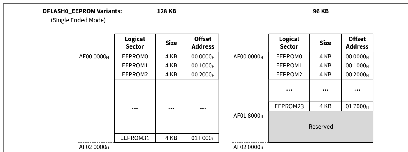
Figure 2 DFlash variants
