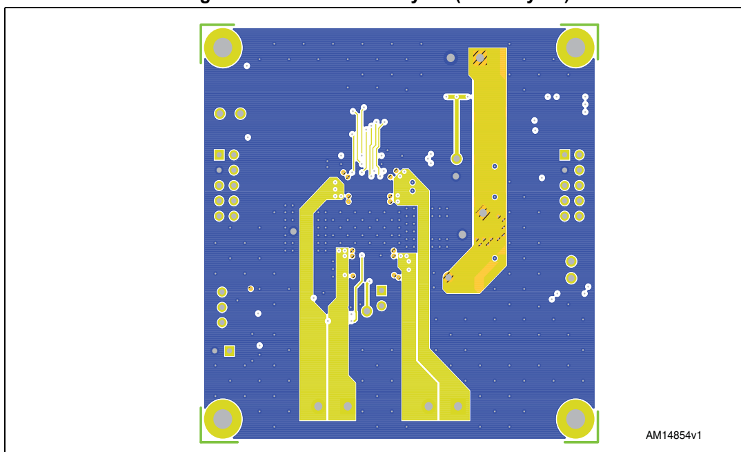
Figure 4. EVAL6472PD - layout (inner layer2)
