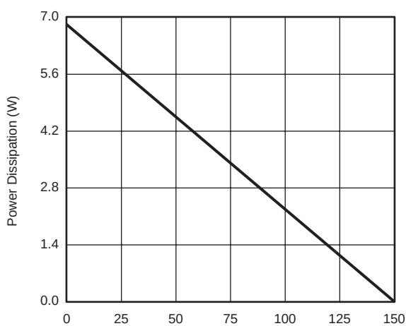
Power, Junction-to-Foot
