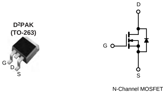
N-Channel MOSFET
