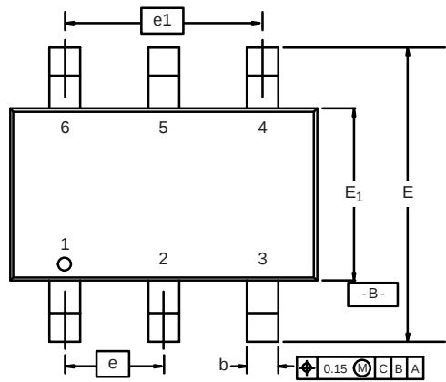
6-LEAD TSOP
