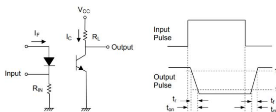
Fig.8 Switching Time Test Circuit & Waveforms
