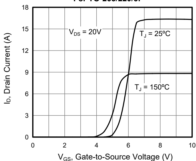
Figure 6. Transfer Characteristics
