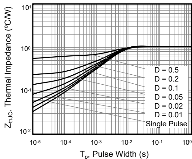
Figure 2. Transient Thermal Impedance For TO-263/220/3P
