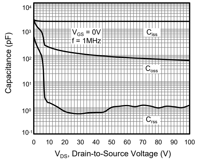
Figure 8. Capacitance
