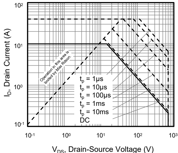
Figure 4. Safe Operation Area For TO-263/220/3P
