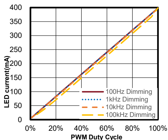
Figure 12.2.a LGS63042, V_{IN}=30V , 3pcs LED Series
