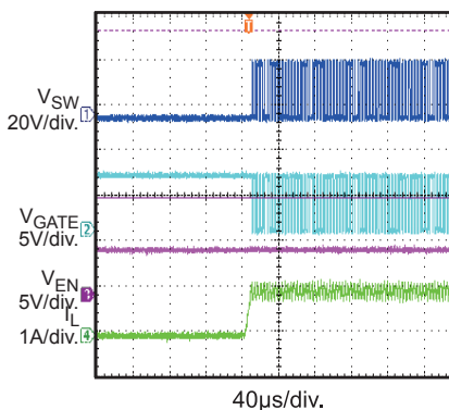
Open LED Load Recovery
