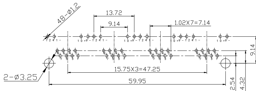
PCB LAYOUT
