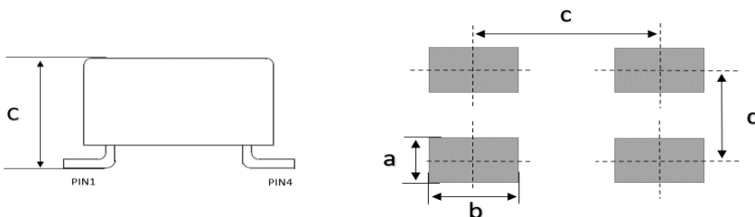
推薦的焊盤尺寸 Recommened Land Pattern
