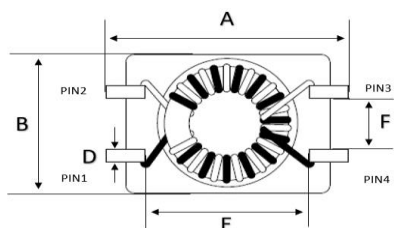
封裝尺寸 Dimension (mm)
