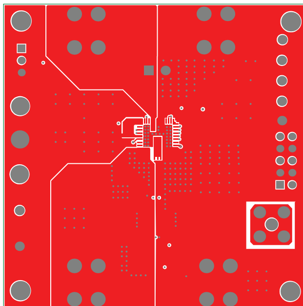
Figure 5: Top Layer
