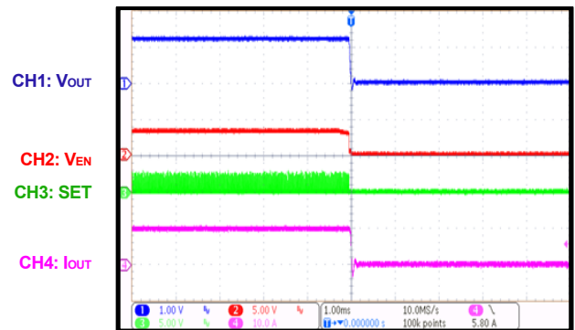
EN Shutdown at Full load
