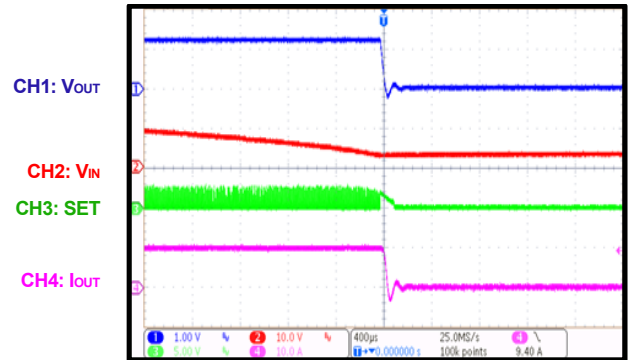
V_{IN} Shutdown at Full load
