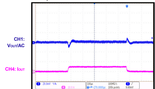
Load Transient @ 0 - 5A Load, 20A/μs
