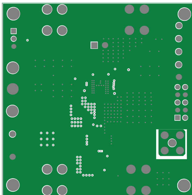
Figure 7: Inner Layer 1
