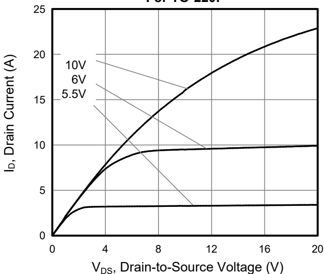
Figure 5. Output Characteristics
