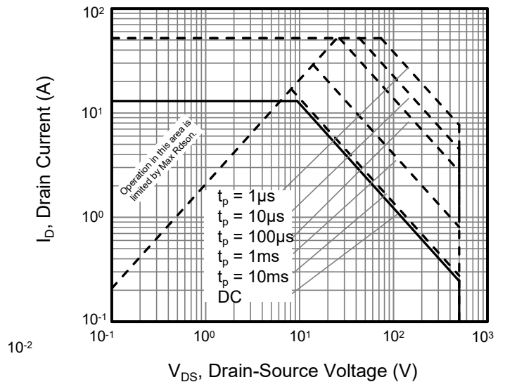
Figure 4. Safe Operation Area For TO-220/3P/247/263
