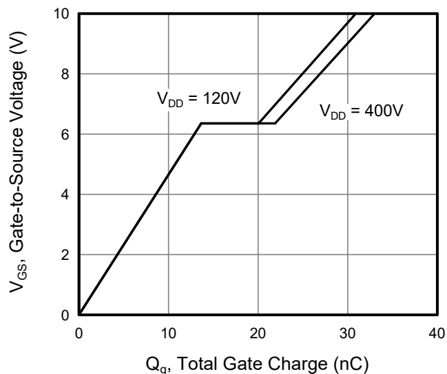
Figure 9. Gate Charge
