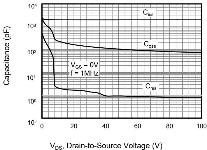
Figure 8. Capacitance
