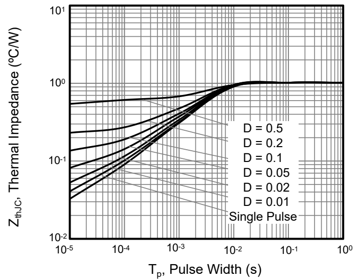
Figure 2. Transient Thermal Impedance For TO-220/3P/247/263
