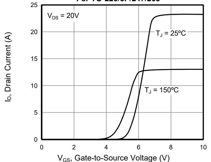
Figure 6. Transfer Characteristics
